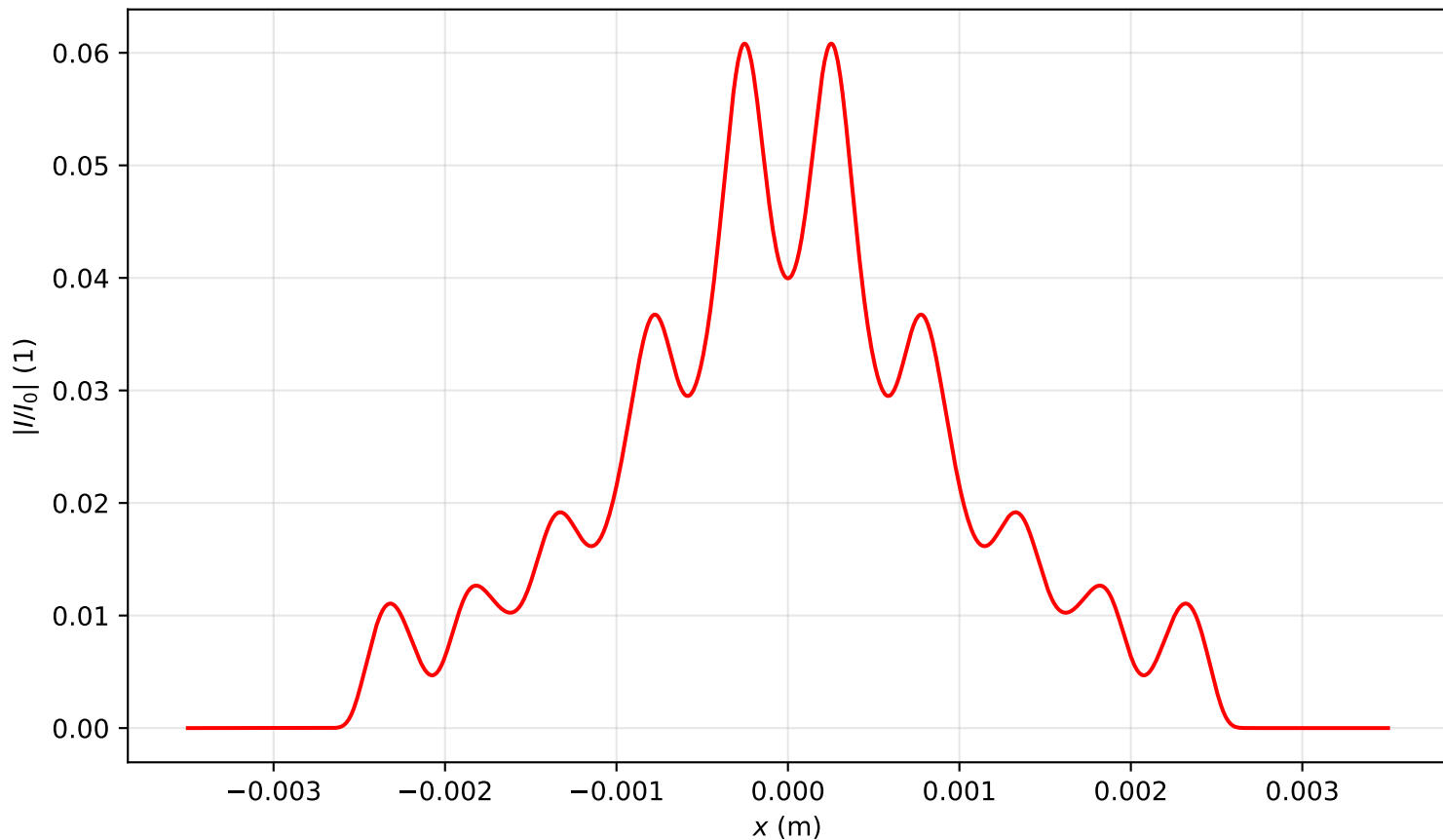
Intensity profile I(x, y = 0, z = 3.662)/I_0 , P_{in}=2.0P_{cr} , artificial time
